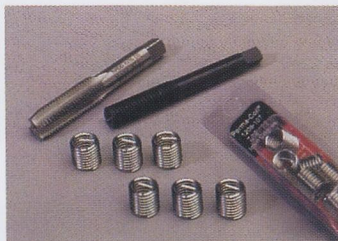
FINE THREAD REPAIR KITS Thread Repair Inserts Tap Insert Prewinder Installation Tool
