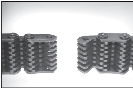
Fig. 4 Separate the two ends.
