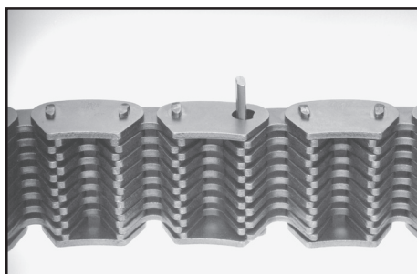
Fig. 7 Lace the joining ends together. (Note the difference in the joining guide link's aperture.) Insert the connecting rocker being careful of orientation. (See Fig. 6 above.)
