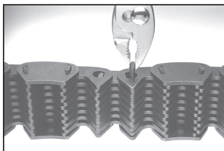
Fig. 4 Remove the two rockers.
