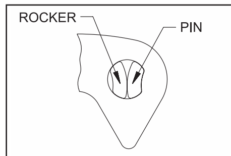
Fig. 6 Note the position and orientation of the pin relative to the rocker. They are designed to roll on each other.
