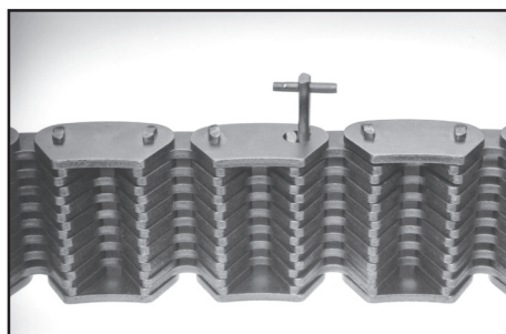
Fig. 8 Insert the connecting pin assembly which consists of a connecting pin and a tapped-in spirol pin. Carefully turn the chain over, and insert the other spirol pin.
