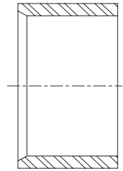
Inner Ring E-XXX-60
