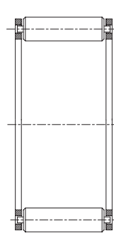
Roller Assembly WS-XXX
