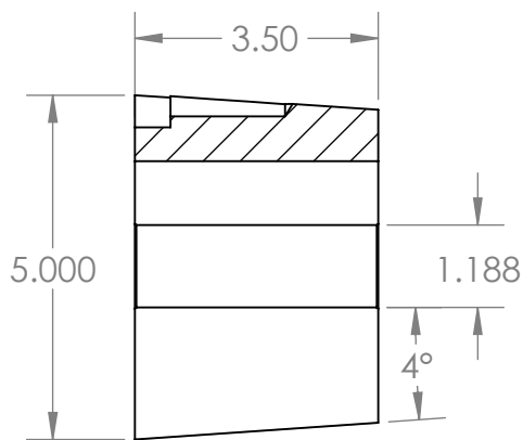
SECTION B-B
