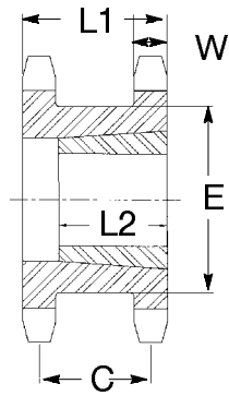
TYPE ATL TAPER-LOCK
