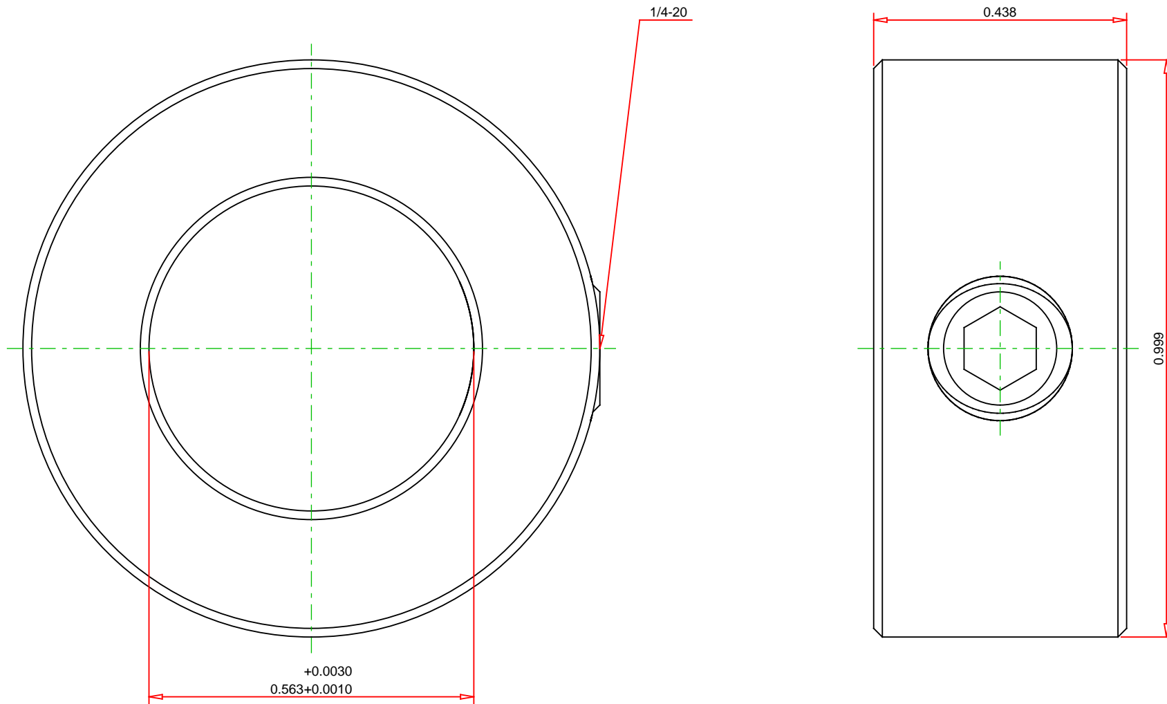
Screw : Hex Socket Set Screw, 3A Thread, Stainless Steel, ASTM F880: 1/4-20 x 1/4
