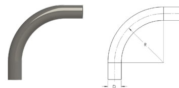
90° Plain End
